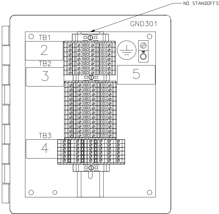
10" x 8" x 6" BACKPANEL LAYOUT
