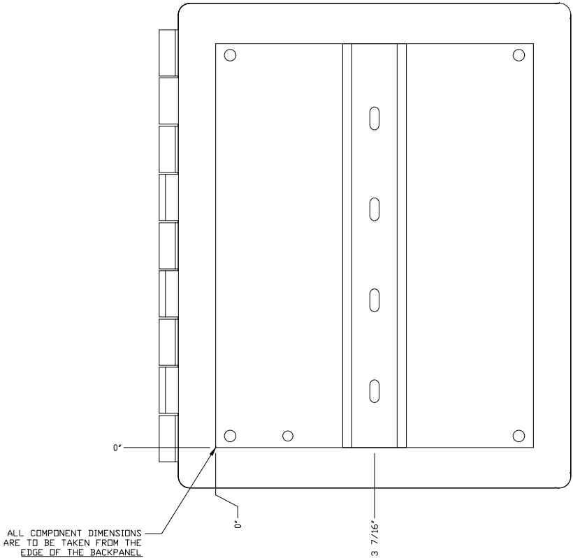
BACKPANEL DETAIL
